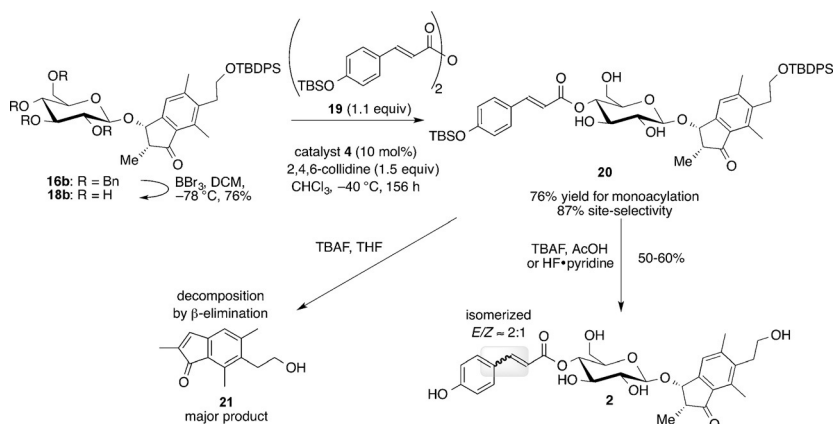
Scheme 3. Problems encountered during the late-stage deprotection toward the total synthesis of 2 . TBAF = tetra- n -butylammonium fluoride.
