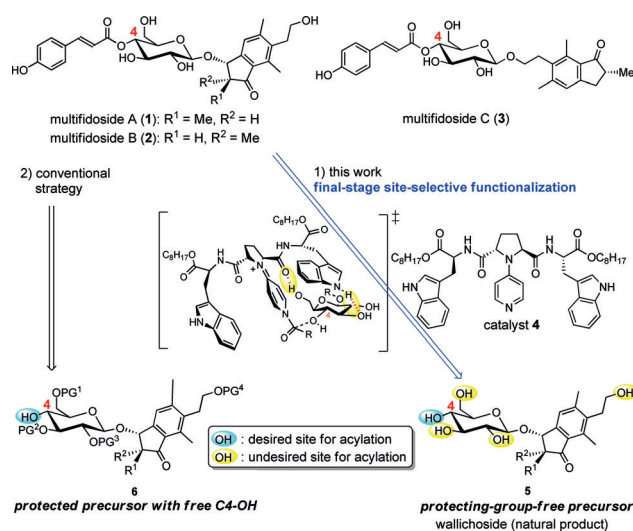
Figure 1. Structures of multifidosides A–C and two synthetic strategies. Route 1 (this work): an organocatalyzed final-stage site-selective acylation of the precursor 5 . Route 2: conventional strategy using the protected precursor 6 . PG = protecting group.
